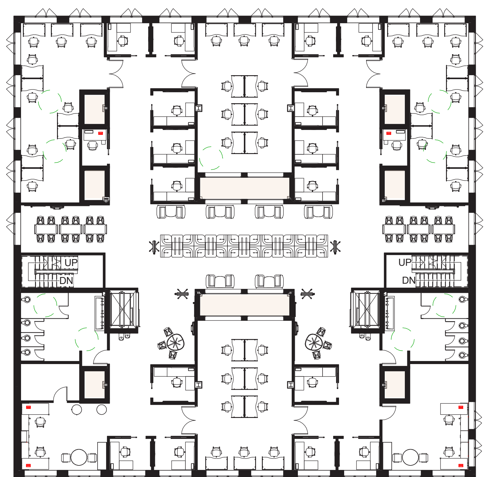
LEVEL 3- FLOOR PLAN
