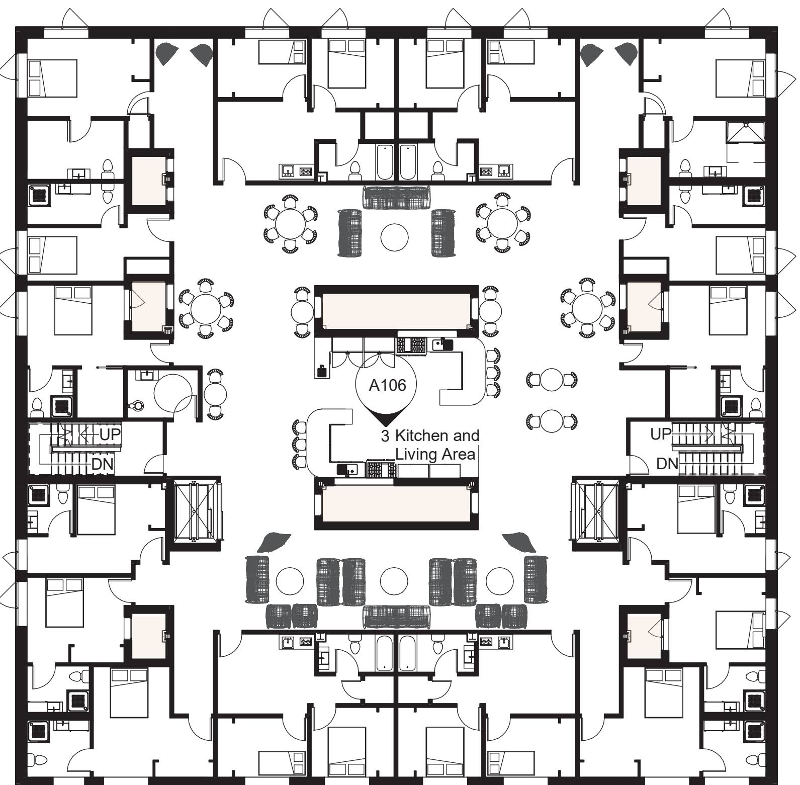
LEVEL 4,5, AND 6- FLOOR PLAN
