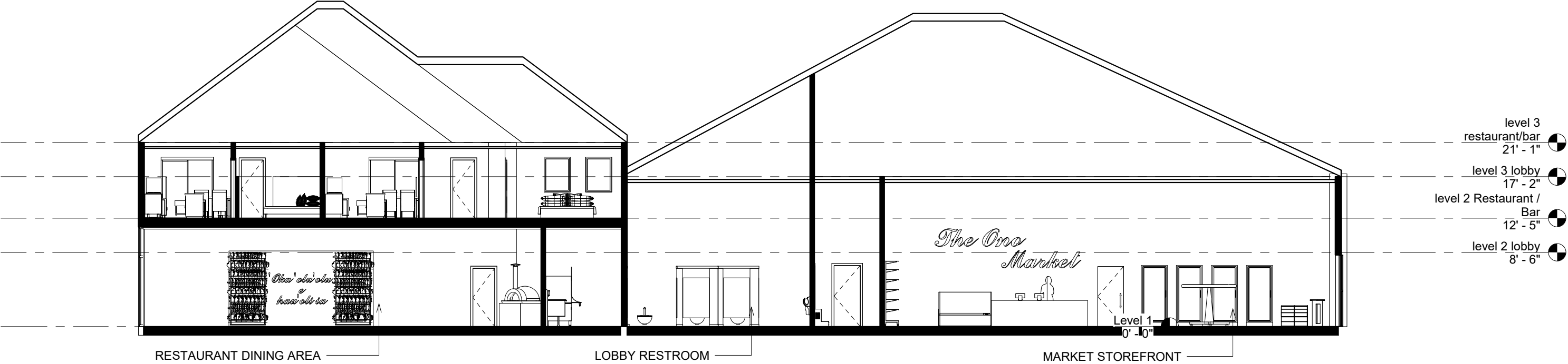
BUILDING SECTION
