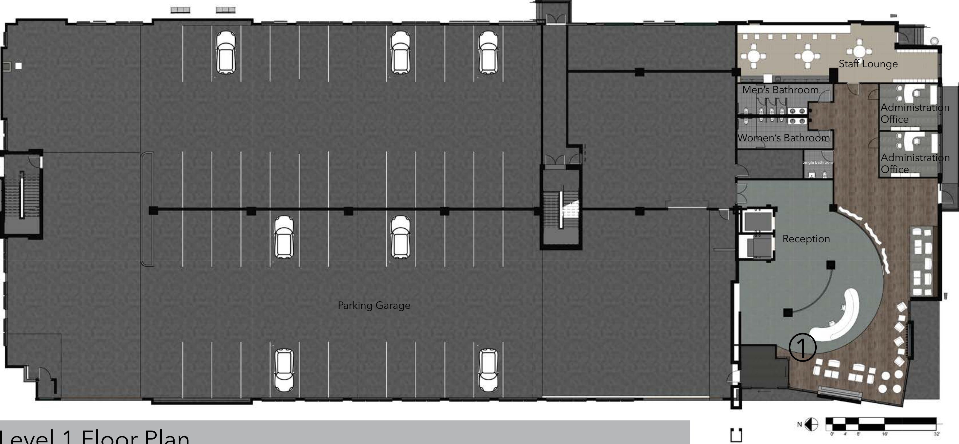
Level 1 Floor Plan
